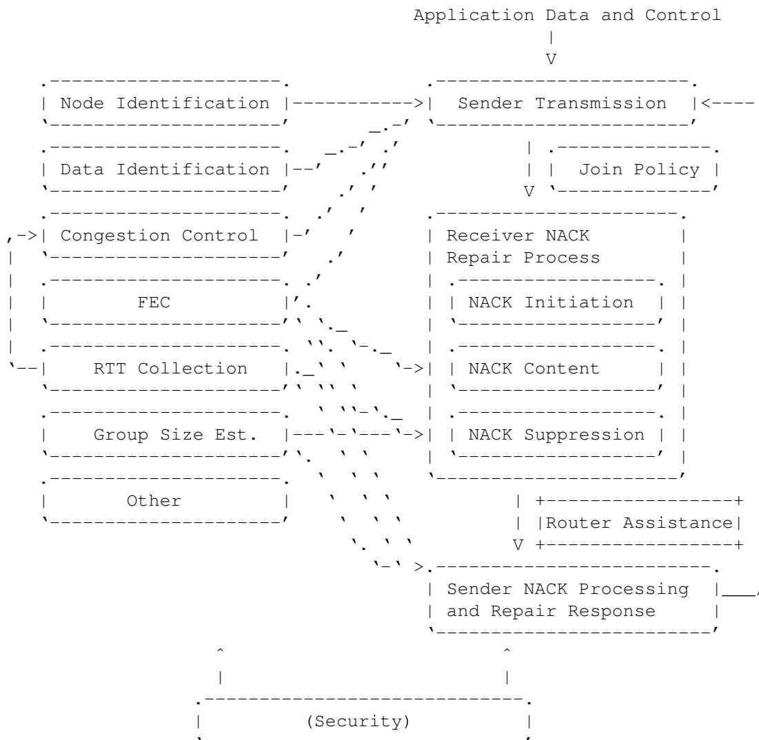
Fig. 1 - NACK-based Reliable Multicast Building Block Framework
