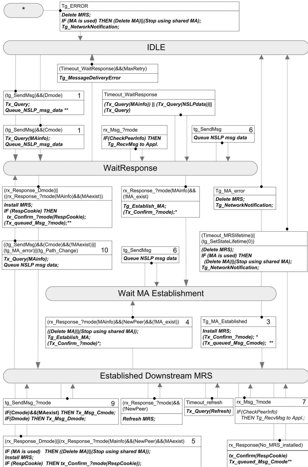
Figure 1: GIST Querying Node State Machine
