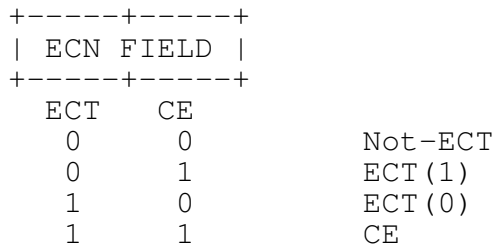
Figure A.2: The ECN Field in IP.
