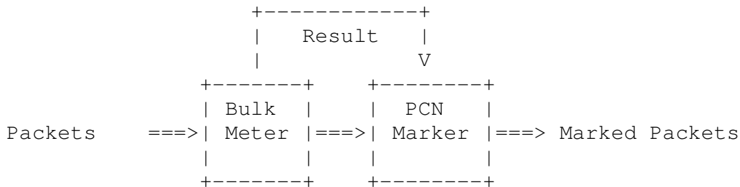
Figure 1: Block Diagram of Meter and Marker Function
