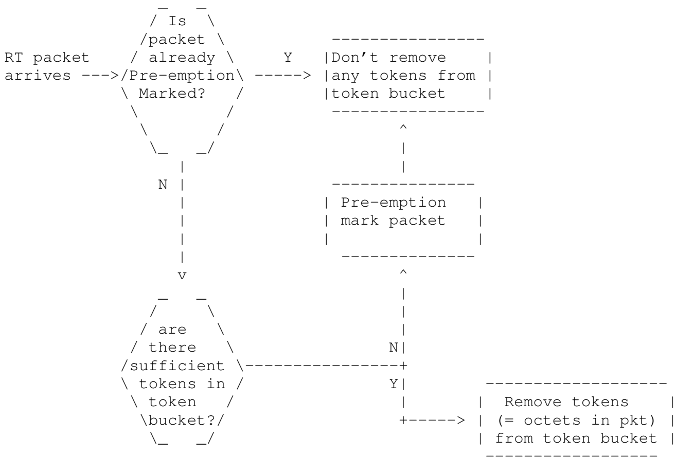
Figure 4: Router action to support pre-emption alerting
