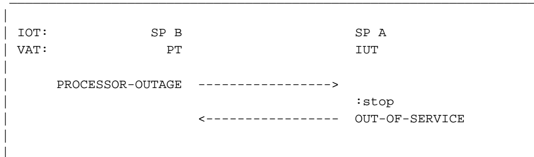
Figure 3.1.31-1. Deactivation during RPO
